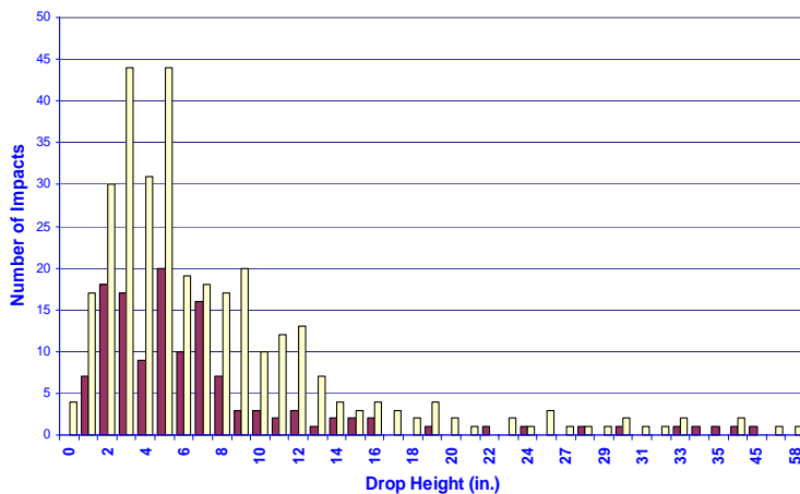
Number of Impacts vs. Drop Height for Route 1051
